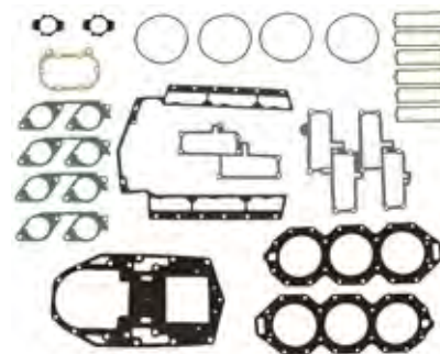
18-4429 POWERHEAD GASKET SET Fits: 200 Ficht FFI (1999-01), 225 (2000-04), 250 (2000-04), 3.3L (2000-04)
