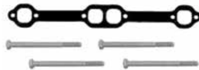
18-8520 EXHAUST MANIFOLD MOUNTING KIT Mercruiser GM Small Block V8 305-350cu.in. (Models: 198, 200, 228, 230, 260, 898) Used with: Manifold: 18-1950-1,18-1951-1, 18-1953-2
