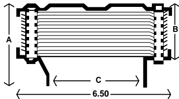
ANODIZED ALUMINUM FLAME ARRESTOR SPECIFICATIONS
