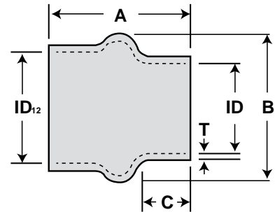
Reducing Hump Hose
